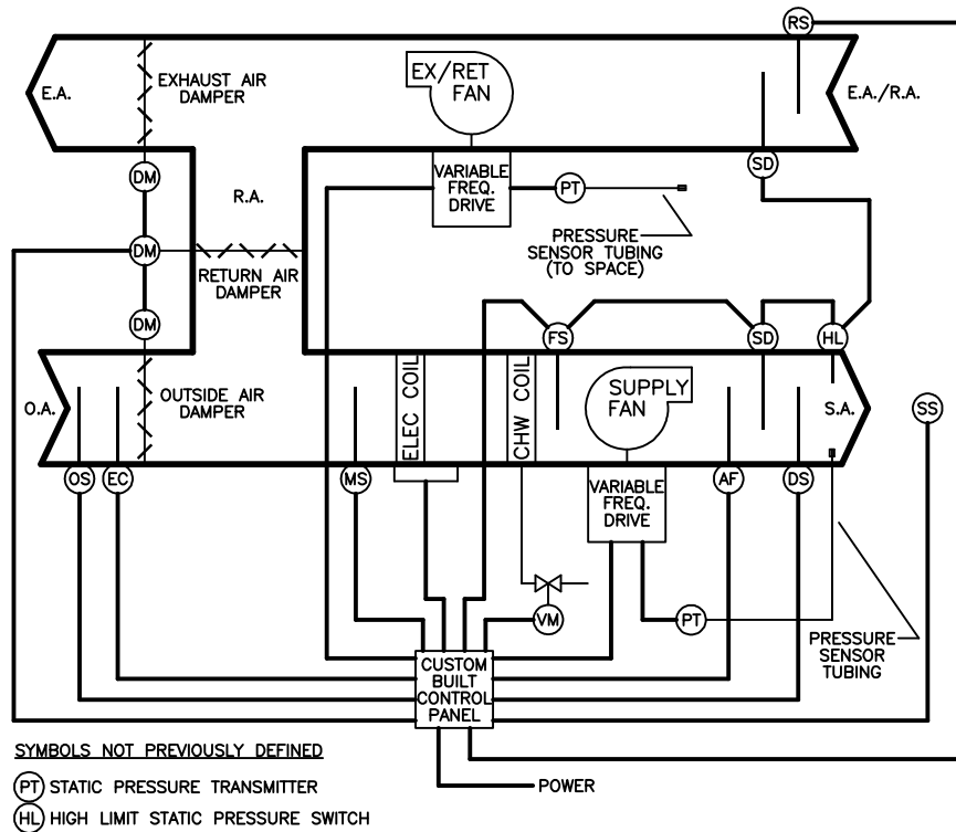
Figure 11.8 VAV air handling unit, electric heating and chilled water cooling, nicely equipped with all the fixings required to blow cold air at a variable rate.
