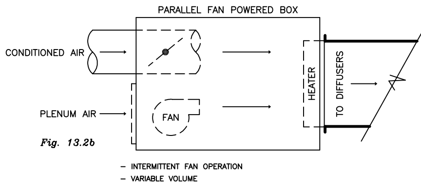
Figures 13.2a & 13.2b Series and parallel fan powered boxes with heat (controllers and actuators not shown).
