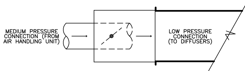
Figure 13.1 Cooling only VAV box (controller and actuator not shown).
